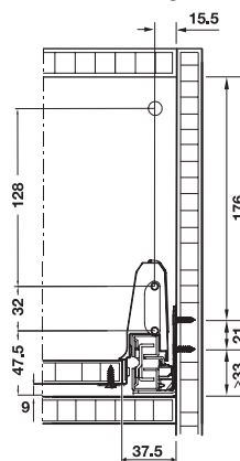
Internal installation height
