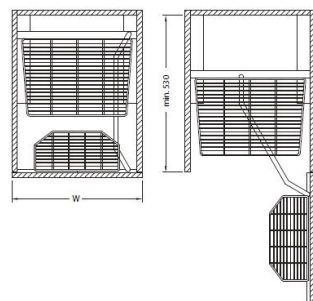
Technical Drawing
