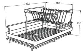
Technical Drawing
