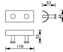
Technical Drawing
