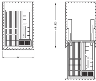
Technical Drawing
