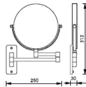
Technical Drawing
