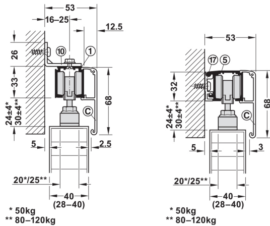
Wall mounting with mounting bracket
