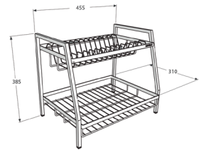
Technical Drawing
