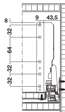
Rear panel installation dimensions
