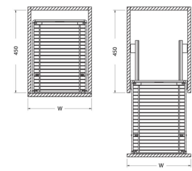
Technical Drawing
